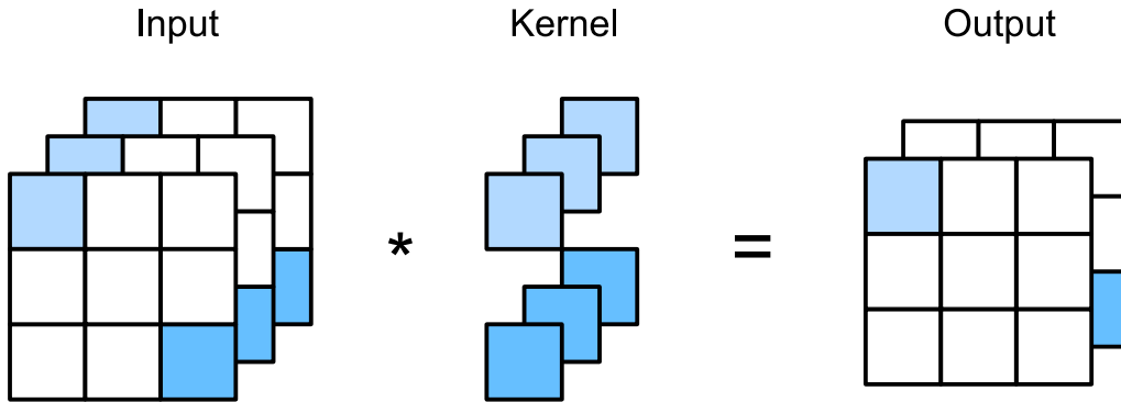
Figure 14.11: Mapping 3 channels to 2 using convolution with a filter of size 1 \times 1 \times 3 \times 2 . Adapted from Figure 6.4.2 of [Zha+20].
