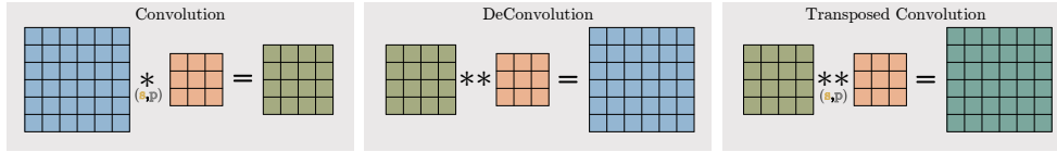
Figure 14.25: Convolution, deconvolution and transposed convolution. Here s is the stride and p is the padding. From https://tinyurl.com/ynxczsut . Used with kind permission of Aqeel Anwar.
