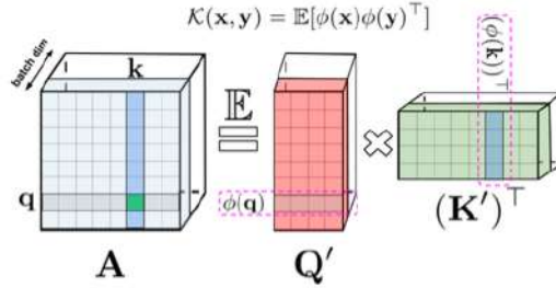
Figure 15.30: Attention matrix \mathbf{A} rewritten as a product of two lower rank matrices \mathbf{Q}' and (\mathbf{K}')^T with random feature maps \phi(\mathbf{q}_i) \in \mathbb{R}^M and \phi(\mathbf{v}_k) \in \mathbb{R}^M for the corresponding queries/keys stored in the rows/columns. Used with kind permission of Krzysztof Choromanski.
