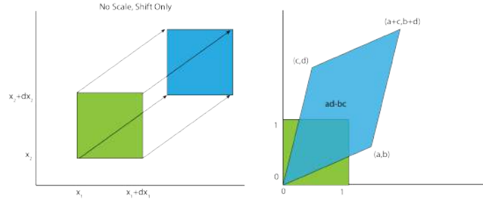
Figure 2.20: Illustration of an affine transformation applied to a unit square, f(x) = Ax + b . (a) Here A = I . (b) Here b = 0 . From [Jan18]. Used with kind permission of Eric Jang.
