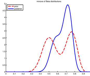
Figure 4.13: A mixture of two Beta distributions. Generated by mixbetademo.ipynb .
