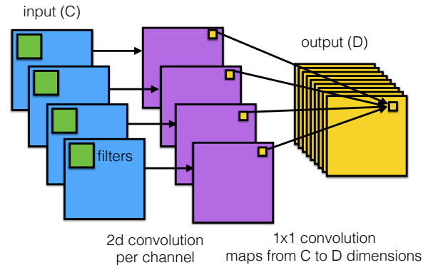
Figure 14.26: Depthwise separable convolutions: each of the C input channels undergoes a 2d convolution to produce C output channels, which get combined pointwise (via 1x1 convolution) to produce D output channels. From https://bit.ly/2L9fm2o . Used with kind permission of Eugenio Culurciello.
