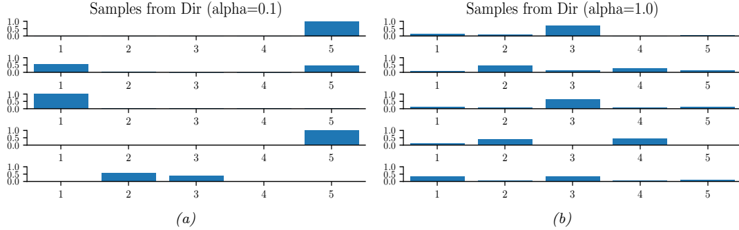
Figure 4.15: Samples from a 5-dimensional symmetric Dirichlet distribution for different parameter values. (a) \tilde{\alpha} = (0.1, \dots, 0.1) . This results in very sparse distributions, with many 0s. (b) \tilde{\alpha} = (1, \dots, 1) . This results in more uniform (and dense) distributions. Generated by dirichlet_samples_plot.ipynb .
