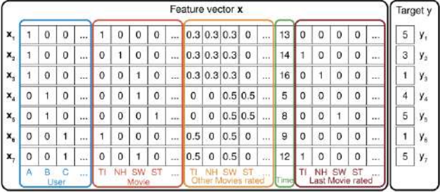
Figure 22.6: Illustration of a design matrix for a movie recommender system, where we show the id of the user and movie, as well as other side information. From Figure 1 of [Ren12]. Used with kind permission of Stefan Rendle.
