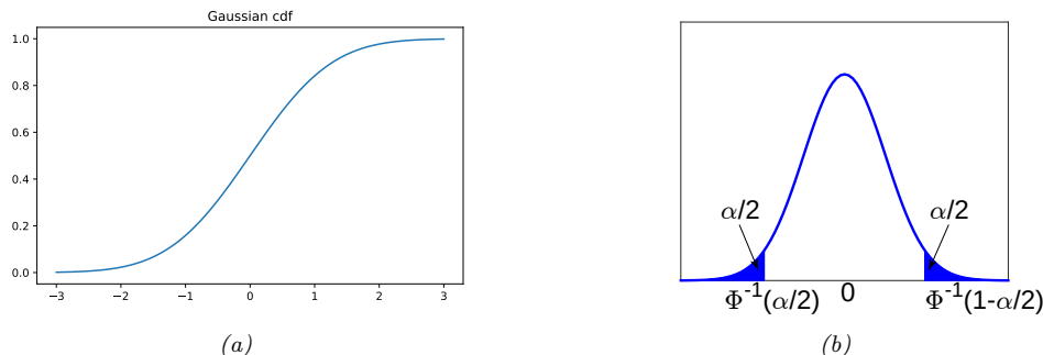
Figure 2.2: (a) Plot of the cdf for the standard normal, \mathcal{N}(0,1) . Generated by gauss_plot.ipynb . (b) Corresponding pdf. The shaded regions each contain \alpha/2 of the probability mass. Therefore the nonshaded region contains 1 - \alpha of the probability mass. The leftmost cutoff point is \Phi^{-1}(\alpha/2) , where \Phi is the cdf of the Gaussian. By symmetry, the rightmost cutoff point is \Phi^{-1}(1 - \alpha/2) = -\Phi^{-1}(\alpha/2) . Generated by quantile_plot.ipynb .
