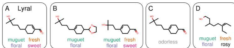
Figure 23.9: Structurally similar molecules do not necessarily have similar odor descriptors. (A) Lyr al, the reference molecule. (B) Molecules with similar structure can share similar odor descriptors. (C) However, a small structural change can render the molecule odorless. (D) Further, large structural changes can leave the odor of the molecule largely unchanged. From Figure 1 of [SL+19], originally from [OPK12]. Used with kind permission of Benjamin Sanchez-Lengeling.
