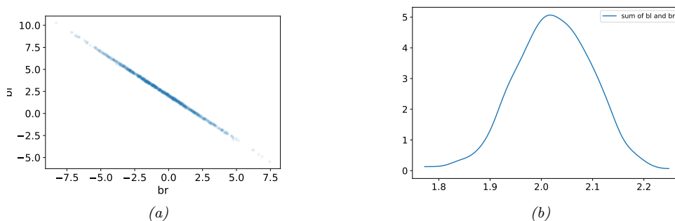
Figure 11.24: Posteriors for the multi-leg example. (a) Joint posterior p(\beta_l, \beta_r | \mathcal{D}) (b) Posterior of p(\beta_l + \beta_r | \mathcal{D}) . Generated by multi_collinear_legs_numpyro.ipynb .
