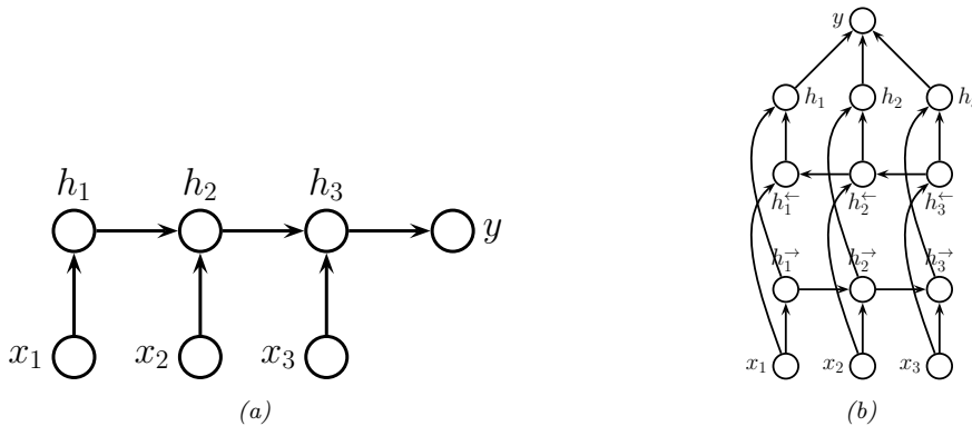
Figure 15.4: (a) RNN for sequence classification. (b) Bi-directional RNN for sequence classification.
