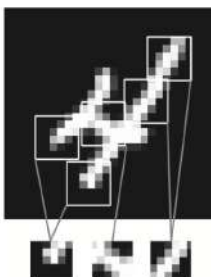
Figure 14.2: We can classify a digit by looking for certain discriminative features (image templates) occurring in the correct (relative) locations. From Figure 5.1 of [Cho17]. Used with kind permission of Francois Chollet.
