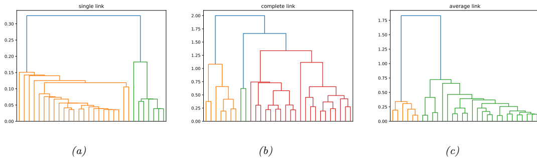
Figure 21.4: Hierarchical clustering of yeast gene expression data. (a) Single linkage. (b) Complete linkage. (c) Average linkage. Generated by hclust_yeast_demo.ipynb .
