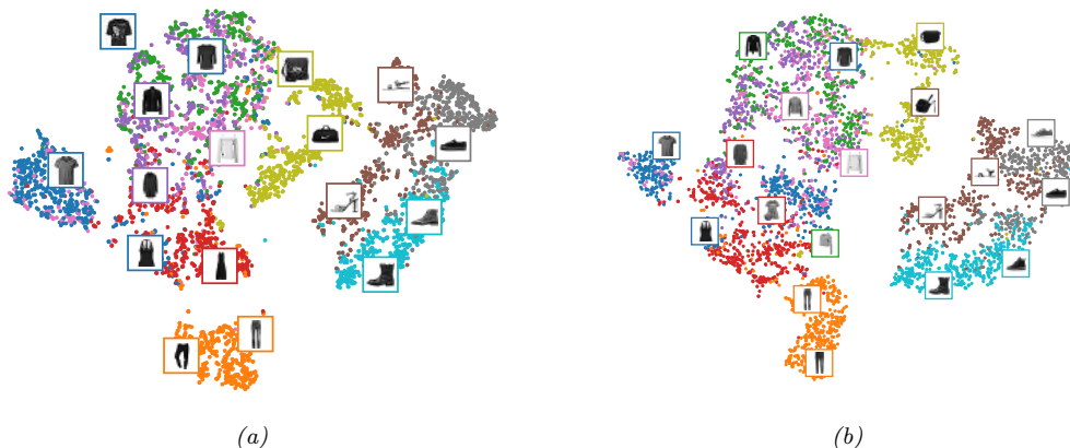
Figure 20.18: tSNE plot of the first 2 latent dimensions of the Fashion MNIST validation set using an autoencoder. (a) MLP. (b) CNN. Adapted from Figure 17.5 of [Gér19]. Generated by ae_mnist_tf.ipynb .
