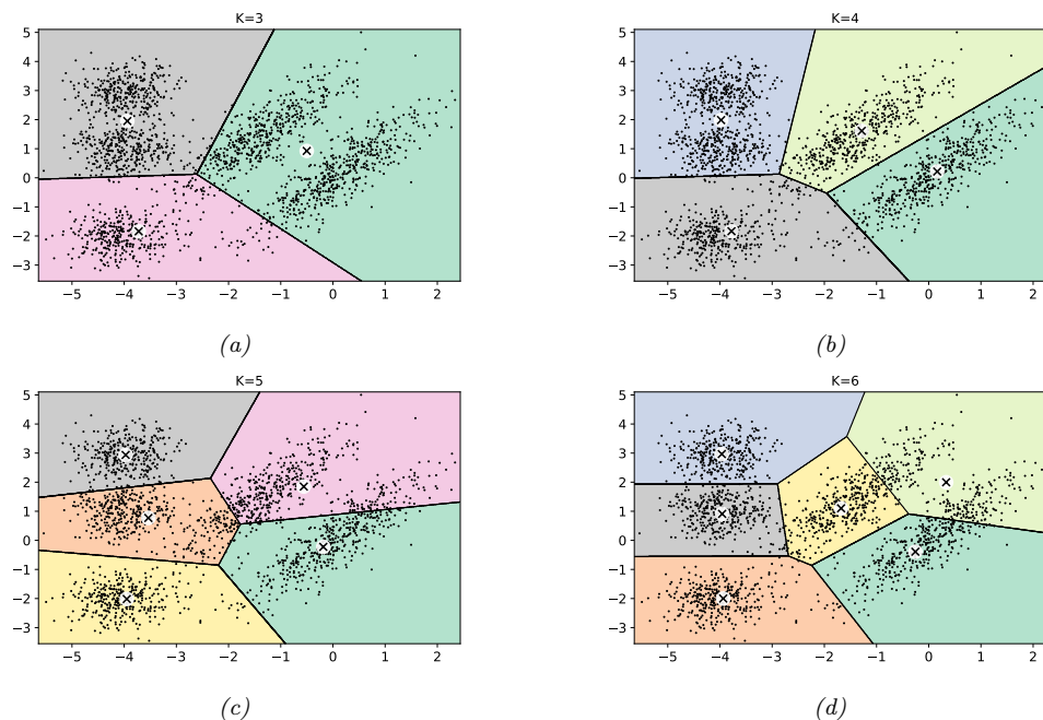
Figure 21.12: Voronoi diagrams for K -means for different K on the 2d dataset from Figure 21.7. Generated by kmeans_silhouette.ipynb .
